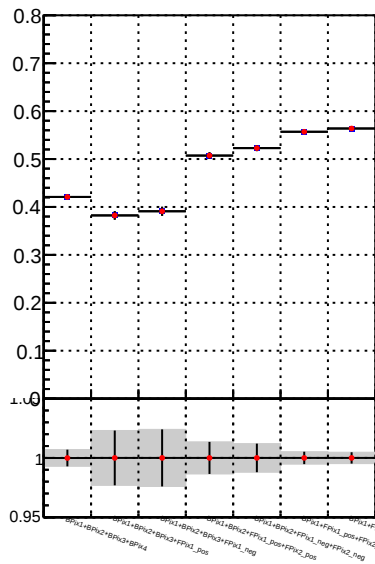
Fake rate vs. DQM_TT_mkFit-DQM_i2 DQM_TT_mkFit-DQM_adjustedi2
