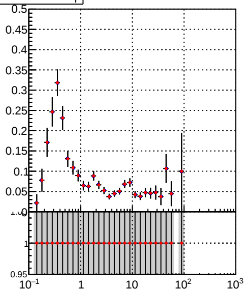
■ DQM_TT_mkFit-DQM_i2 ● DQM_TT_mkFit-DQM_adjustedI2
