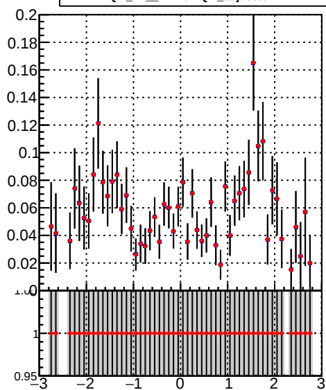
■ DQM_TT_mkFit-DQM_i2 ● DQM_TT_mkFit-DQM_adjustedI2
