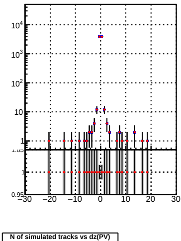
N of simulated tracks vs dz(PV) zoomed in
