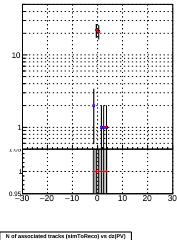
N of associated tracks (simToReco) vs dz(PV) zoomed in
