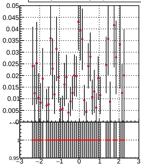
DQM_TT_mkFit-DQM_i2 DQM_TT_mkFit-DQM_adjustedI2
