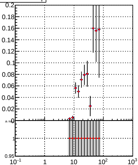
DQM_TT_mkFit-DQM_i2 DQM_TT_mkFit-DQM_adjustedI2
