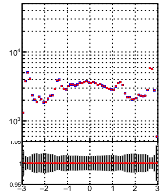
—•— DQM_TT_mkFit-DQM_i2 —•— DQM_TT_mkFit-DQM_adjustedi2
