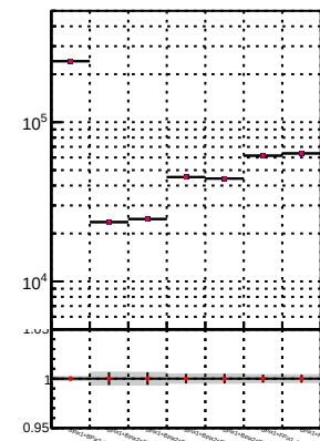
N of reco track vs. \chi^2 for DQM TT mkFit-DQM i2 and DQM TT mkFit-DQM adjustedi2
