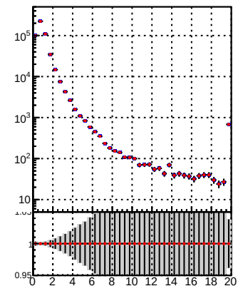
N of reco track vs. \chi^2 for DQM TT mkFit-DQM i2 and DQM TT mkFit-DQM adjustedi2
