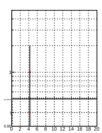
N of reco track vs. \chi^2 for DQM TT and mkFit-DQM i2
