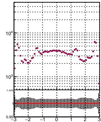
N of reco track vs \eta Legend: DQM TT mkFit-DQM i2 (blue line with dots) DQM TT mkFit-DQM adjustedi2 (red line with dots)
