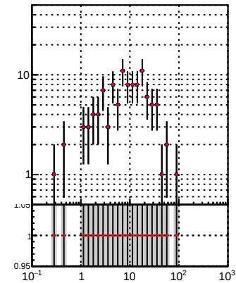
—•— DQM_TT_mkFit-DQM_i2 —•— DQM_TT_mkFit-DQM_adjusted2
