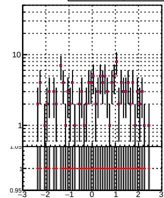
—•— DQM_TT_mkFit-DQM_i2 —•— DQM_TT_mkFit-DQM_adjusted2
