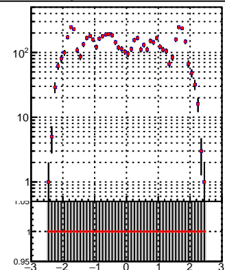
N of reco track vs \eta —●— DQM_TT_mkFit-DQM_j2 —●— DQM_TT_mkFit-DQM_adjusted2
