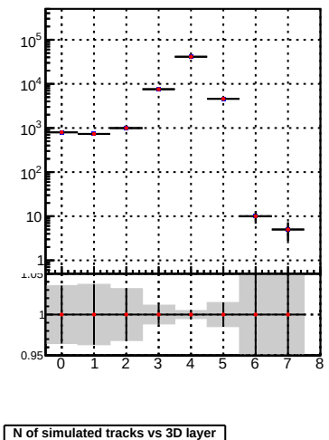
N of simulated tracks vs 3D layer
