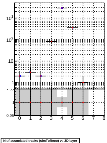
N of associated tracks (simToReco) vs 3D layer
