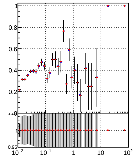
█ DQM_TT_mkFit-DQM_i2 █ DQM_TT_mkFit-DQM_adjusted2
