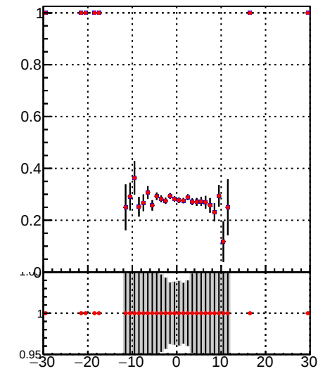
█ DQM_TT_mkFit-DQM_i2 █ DQM_TT_mkFit-DQM_adjusted2
