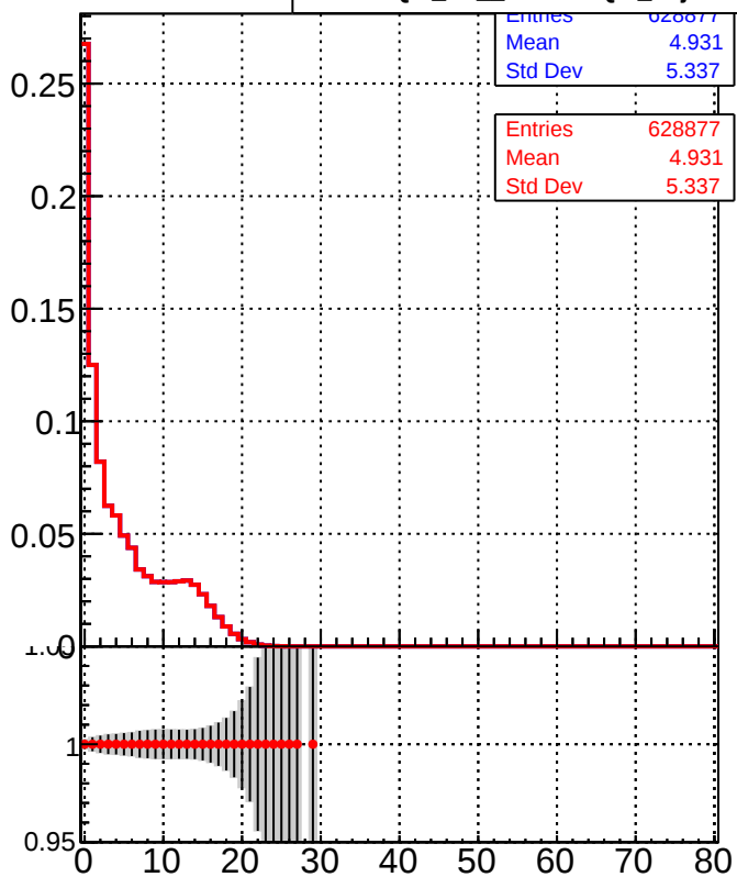
— DQM_TT_mkFit-DQM_i2 — DQM_TT_mkFit-DQM_adjusted_i2
