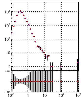
—●— DQM_TT_mkFit-DQM_j2 —●— DQM_TT_mkFit-DQM_adjusted2
