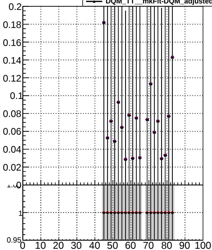
DQM_TT_mkFit-DQM_ DQM_TT_mkFit-DQM_adjusted DQM_TT_mkFit-DQM_adjusted2
