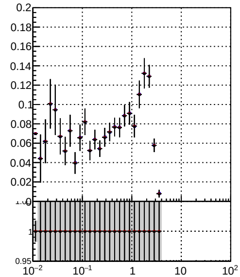
Efficiency vs vertpos Legend: DQM_TT_mkFit-DQM_ (blue line with markers) DQM_TT_mkFit-DQM_adjusted (red line with markers) DQM_TT_mkFit-DQM_adjusted2 (black line with markers)
