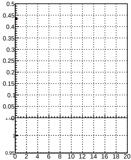
Duplicates Rate vs. \chi^2 adjusted
