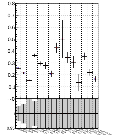
Fake rate vs. DOM TT mkFit-DOM + + + + + + + + + adjusted adjusted2
