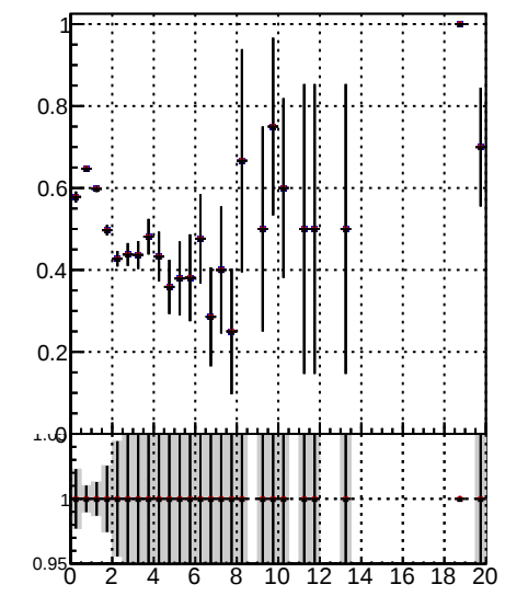
Fake rate vs. DOM TT mkFit-DOM + + + + + + + + + adjusted adjusted2
