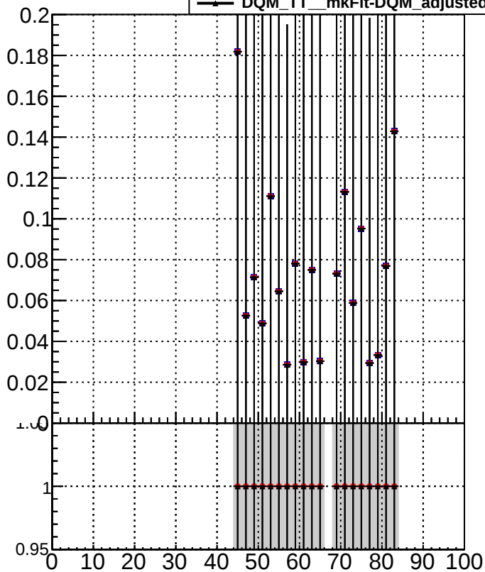
—■ DQM_TT_mkFit-DQM_
