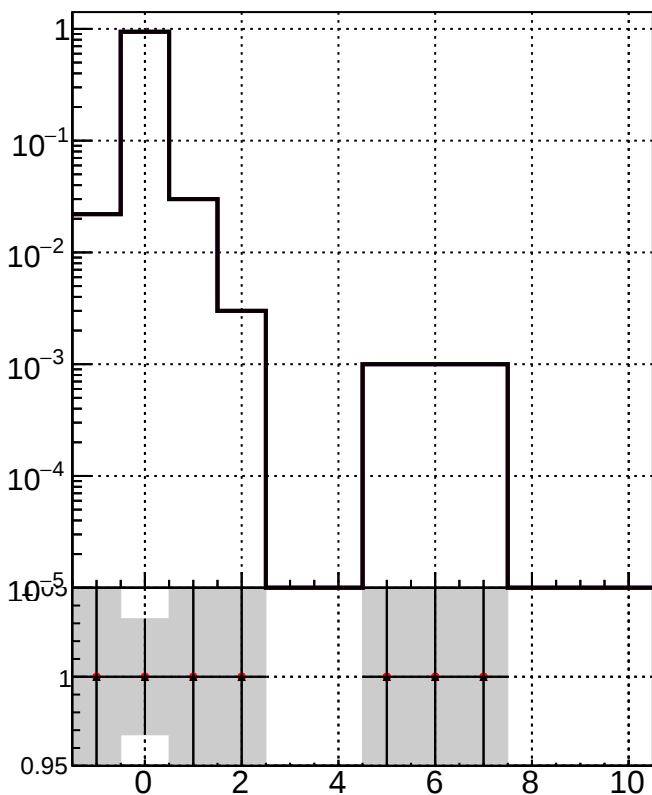
TruePVLocationIndexInRecoVertexCollection
