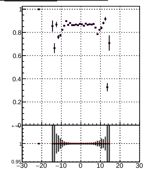
Fake rate vs d Legend: DOM TT mkFit-DOM DOM TT mkFit-DOM-adjusted DOM TT mkFit-DOM-adjusted2
