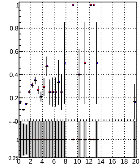
Fake rate vs. \chi^2 for DOM TT mkFit-DOM adjusted and DOM TT mkFit-DOM adjustedi2
