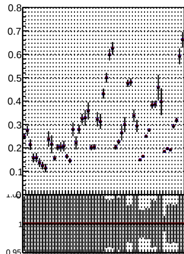
Fake rate vs. — DOM TT mkFit-DOM — DOM TT mkFit-DOM adjusted — DOM TT mkFit-DOM adjusted2
