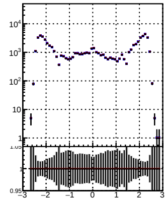
N of reco track vs \eta Legend: BQM TT mkFit-BQM BQM TT mkFit-BQM adjusted2
