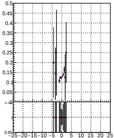
Fake rate vs d —•— DOM TT mkFit-DOM —•— DOM TT mkFit-DOM adjusted —•— DOM TT mkFit-DOM adjusted 12
