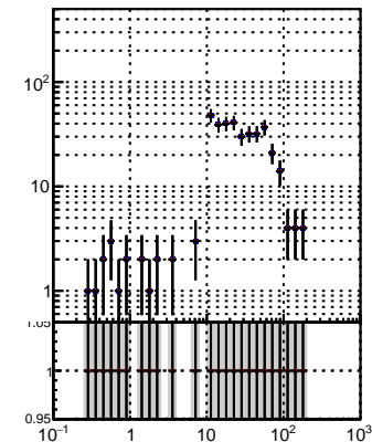
it-BQM-adjusted i2
