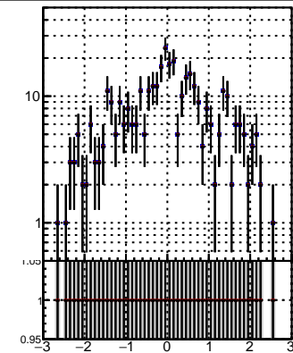
it-BQM-adjusted i2
