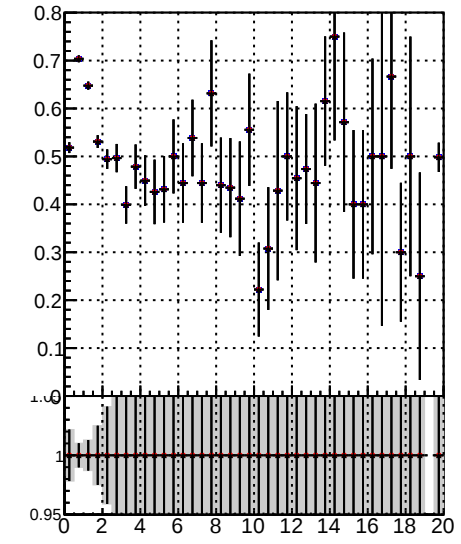
Fake rate vs. \chi^2 for \text{DOM TT mkFit-DOM} , \text{DOM TT mkFit-DOM adjusted} , \text{DOM TT mkFit-DOM adjusted}_2
