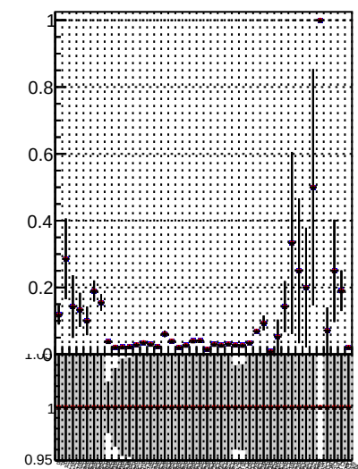
Fake rate vs. DOM TT mkFit-DOM DOM TT mkFit-DOM adjusted DOM TT mkFit-DOM adjusted2
