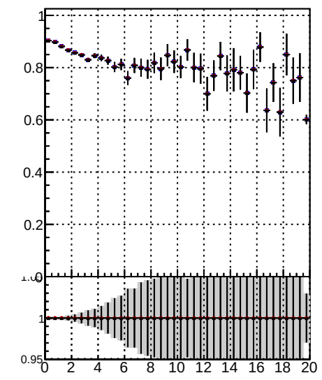
Fake rate vs. DOM TT mkFit-DOM DOM TT mkFit-DOM adjusted DOM TT mkFit-DOM adjusted2
