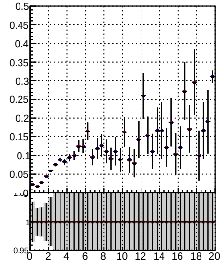
Fake rate vs. DOM TT mkFit-DOM DOM TT mkFit-DOM adjusted DOM TT mkFit-DOM adjusted2
