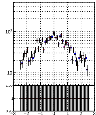
N of reco track vs \eta DQM TT mkFit-DQM adjusted DQM TT mkFit-DQM adjusted 2
