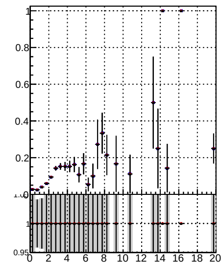
Fake rate vs. \chi^2 for different categories
