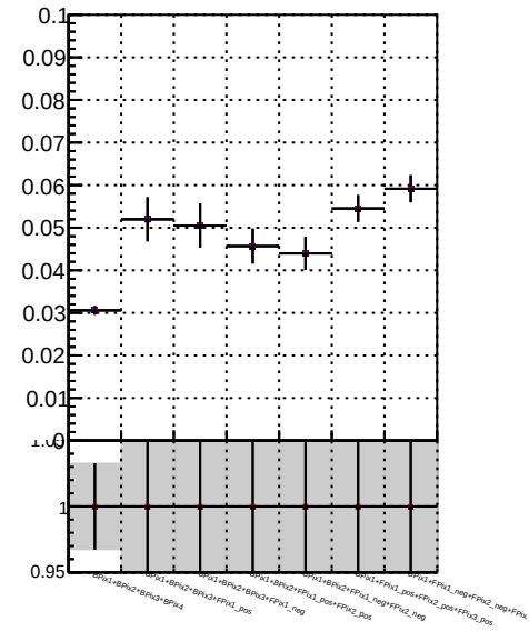
Fake rate vs. \chi^2 for different categories
