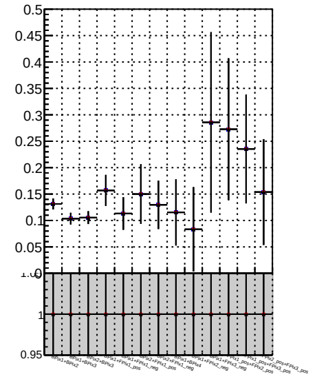
Fake rate vs. DOM TT mkFit-DOM DOM TT mkFit-DOM adjusted DOM TT mkFit-DOM adjustedi2
