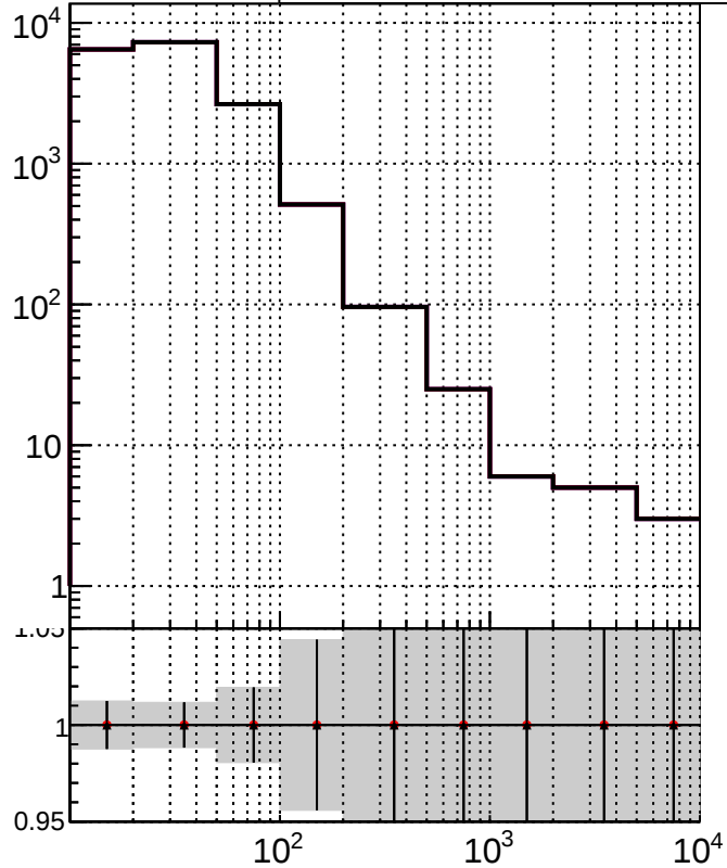
RecoAssoc2GenPVMatched_Pt2
