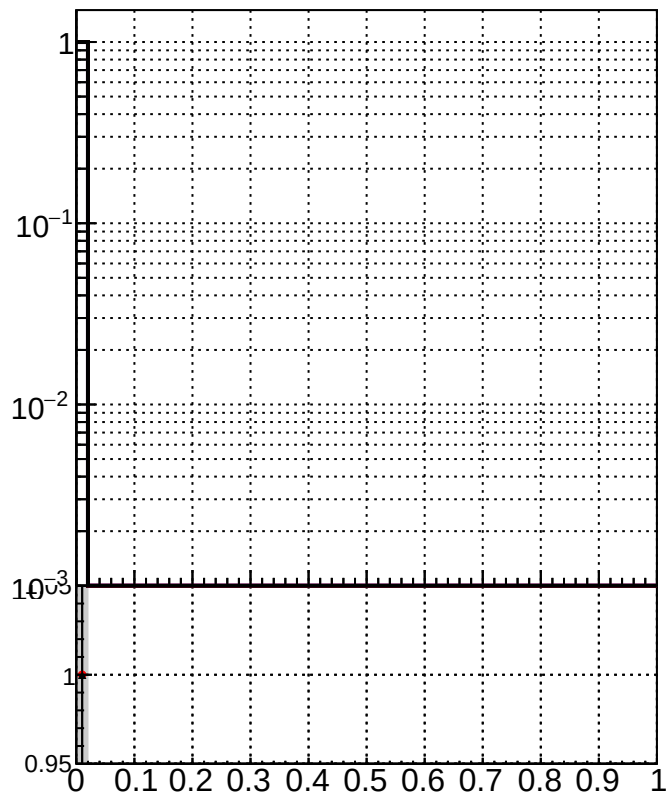
RecoPVAssoc2GenPVNotMatched_Purity
