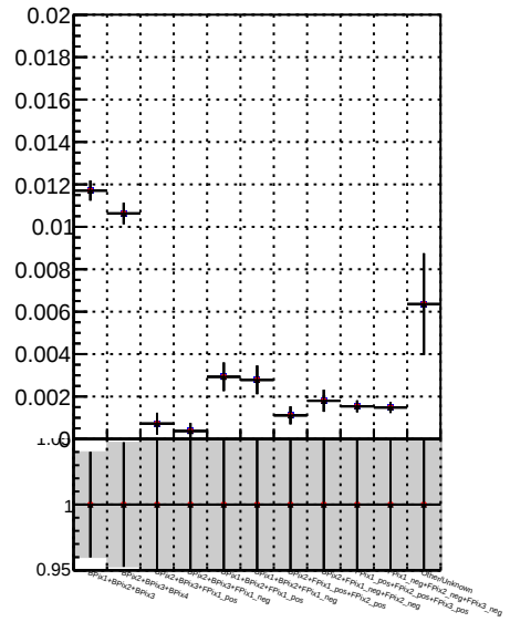
Fake rate vs. DOM TT mkFit-DOM BCOM TT mkFit-DOM adjusted BCOM TT mkFit-DOM adjusted 2
