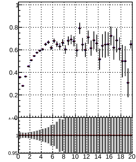
Fake rate vs. DOM TT mkFit-DOM BCOM TT mkFit-DOM adjusted BCOM TT mkFit-DOM adjusted 2
