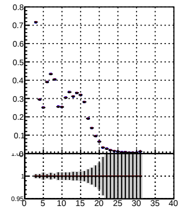
Fake rate vs hit Legend: DQM_TT_mkFit-DQM_ (blue line with dots) DQM_TT_mkFit-DQM_adjusted (red line with dots) DQM_TT_mkFit-DQM_adjusted2 (black line with dots)
