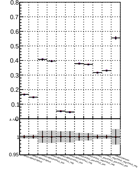
Fake rate vs. DOM TT mkFit-DOM BOM TT mkFit-BOM BOM TT mkFit-BOM adjusted BOM TT mkFit-BOM adjusted2
