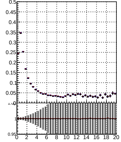
Fake rate vs. DOM TT mkFit-DOM BOM TT mkFit-BOM BOM TT mkFit-BOM adjusted BOM TT mkFit-BOM adjusted2
