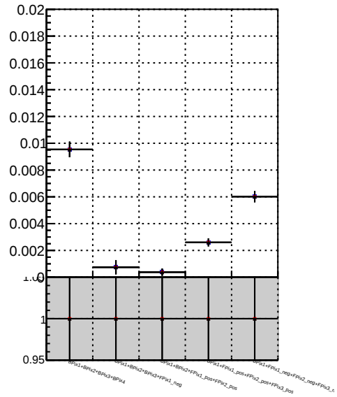
Fake rate vs. — DOM TT mkFit-DOM adjusted — BQM TT mkFit-DOM adjusted — BQM TT mkFit-DOM adjusted 2
