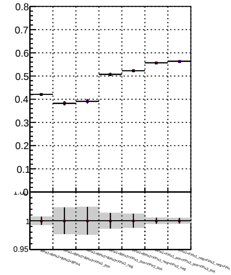
Fake rate vs. — DOM TT mkFit-DOM adjusted — BQM TT mkFit-DOM adjusted — BQM TT mkFit-DOM adjusted 2
