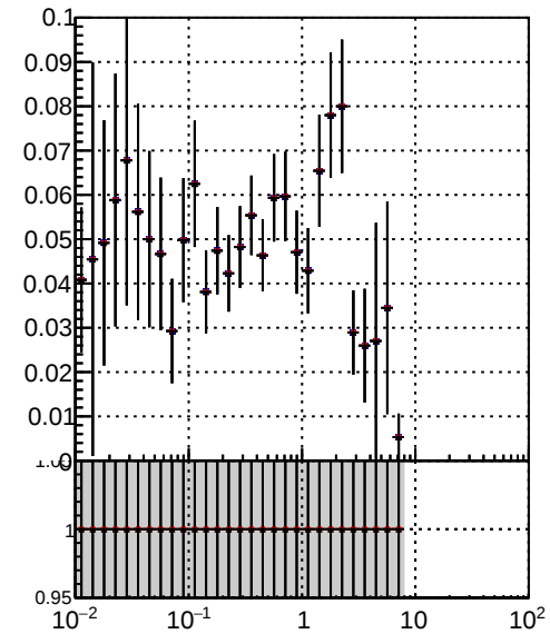
Efficiency vs. \sqrt{s}
