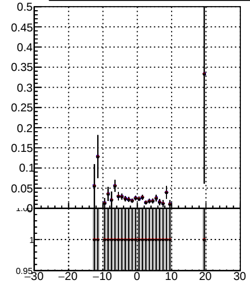
Efficiency vs. \sqrt{s}
