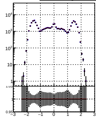
N of reco track vs \eta DOM TT mkFit-DQM adjusted DOM TT mkFit-DQM adjusted2
