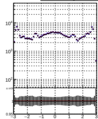
N of reco track vs \eta Legend: BQM TT mkFit-BQM (solid line) BQM TT mkFit-BQM adjusted2 (dashed line)
