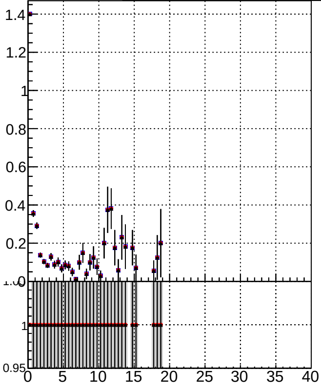
K_S^0 tracking fake rate vs p_T (Detailed View) DQM_TT_mkFit-DQM_ DQM_TT_mkFit-DQM_adjusted DQM_TT_mkFit-DQM_adjusted2
