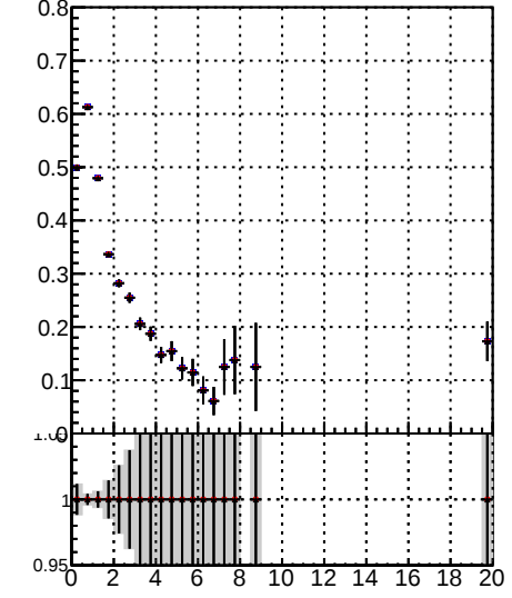
Fake rate vs. \chi^2 for different models and fits. The legend indicates: DOM TT mkFit-DOM (blue), DOM TT mkFit-DOM-adjusted (red), DOM TT mkFit-DOM-adjusted2 (black).
