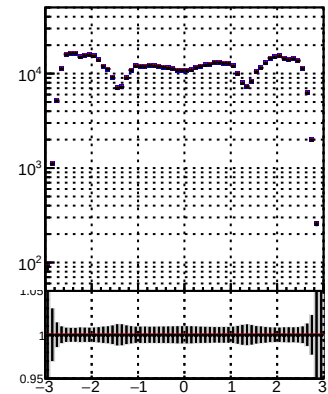
N of reco track vs \eta BQM TT mkFit-BQM BQM TT mkFit-BQM adjusted BQM adjusted2
