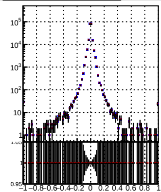
—•— DOM TT mkFit-DQM —•— DOM TT mkFit-DQM adjusted —•— DOM TT mkFit-DQM adjustedi2
