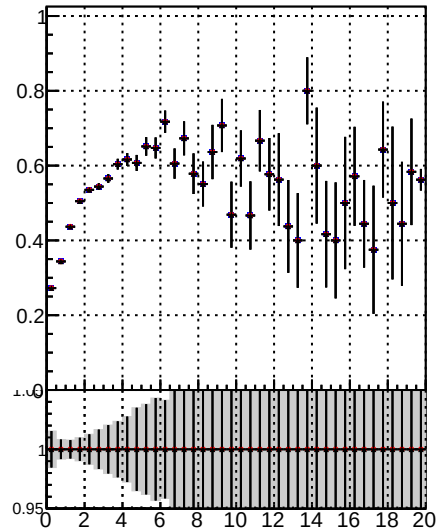
Fake rate vs. \chi^2 adjusted
