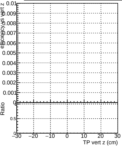
Efficiency vs TP vert z (cm) Legend: DQM_V0001_R0000000001_Global_CMSSW_ckfPU50_RECO DQM_V0001_R0000000001_Global_CMSSW_mkFitPU50LowPtQuad_RECO DQM_V0001_R0000000001_Global_CMSSW_LowptQnoclean_RECO
