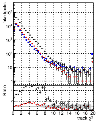
Global CMSSW mkFitPU50_Quad_RECO
