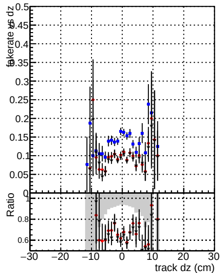
Fake rate vs dz Legend: DOM V0001 R0000000001 Global CMSSW ckfPU50 RECO DOM V0001 R0000000001 Global CMSSW InFPU50LowPtQuad RECO DOM V0001 R0000000001 Global CMSSW LowPtOnoclean RECO
