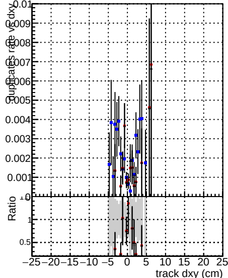
DOM V0001 R0000000001 Global CMSSW ckfPU50 RECO DOM V0001 R0000000001 Global CMSSW InkFPU50L owPtQuad RECO DOM V0001 R0000000001 Global CMSSW LowPtOnoclean RECO
