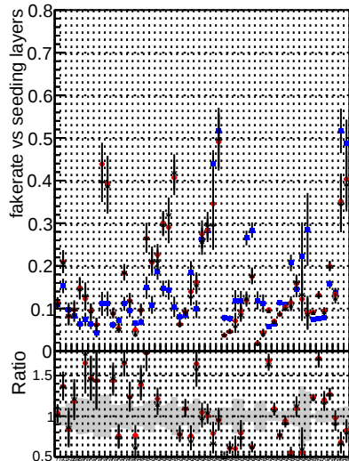
Fake rate vs. DOM V0001 R0000000001 Global CMSSW ckfpu50 RECO DOM V0001 R0000000001 Global CMSSW InFIRPU50LowPtQuad RECO DOM V0001 R0000000001 Global CMSSW LowPtOnoclean RECO
