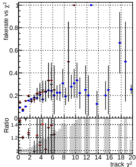
Fake rate vs. DOM V0001 R0000000001 Global CMSSW ckfpu50 RECO DOM V0001 R0000000001 Global CMSSW InFIRPU50LowPtQuad RECO DOM V0001 R0000000001 Global CMSSW LowPtOnoclean RECO
